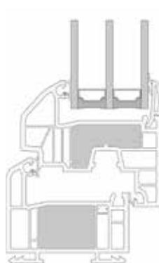
POLYURETHANE FOAM
